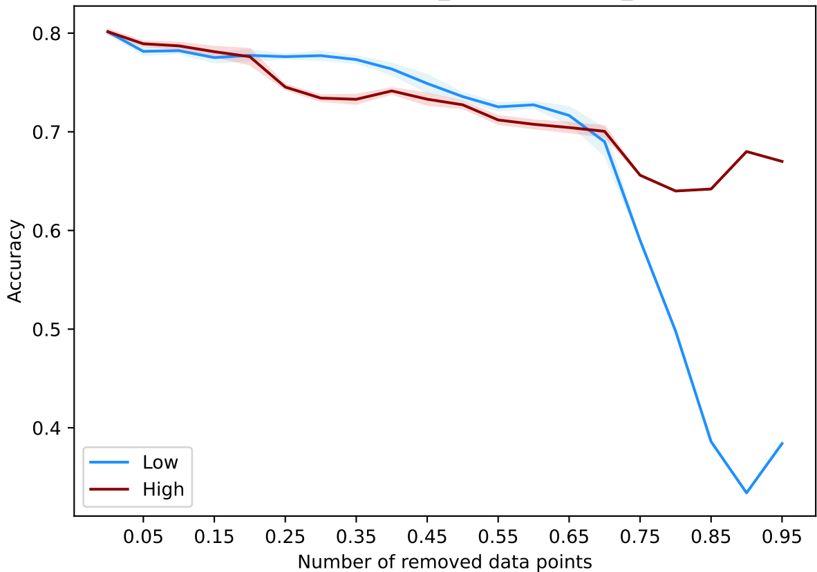
PruningOptimization(optimization_type=size, only_size=100) - adult
